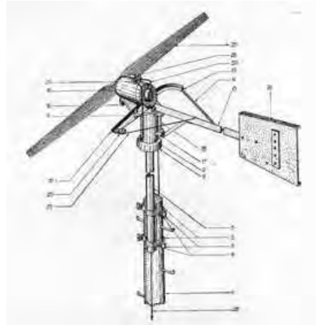
Aerogenerators
