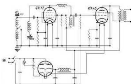
Vefar 2MLD/34
